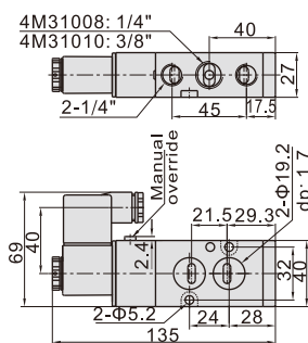
4M310(Terminal)
