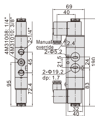
4M320(Terminal)
