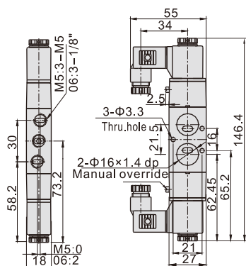
4M120(Terminal)
