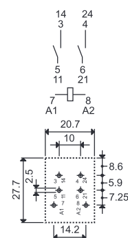
56.42-0300 Copper side view
